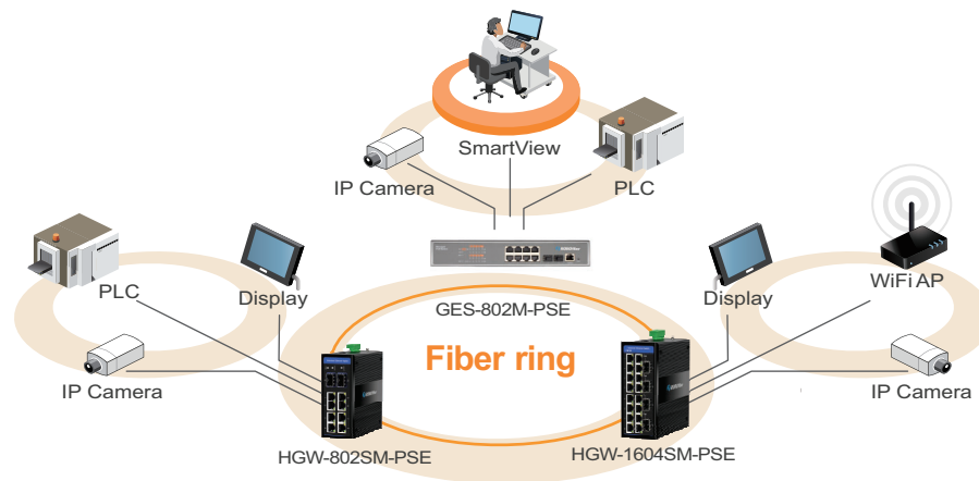
GES-802M Gigabit Ethernet Managed Switch Application
