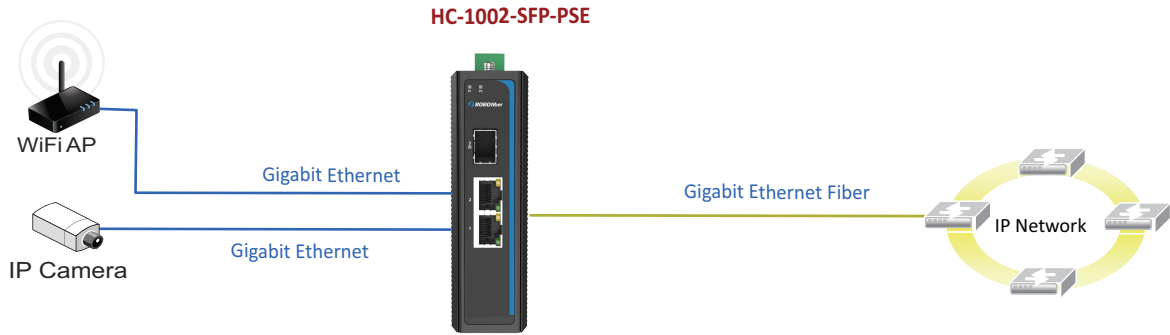
HC-1002-SFP-PSE Gigabit Ethernet Switch Application
