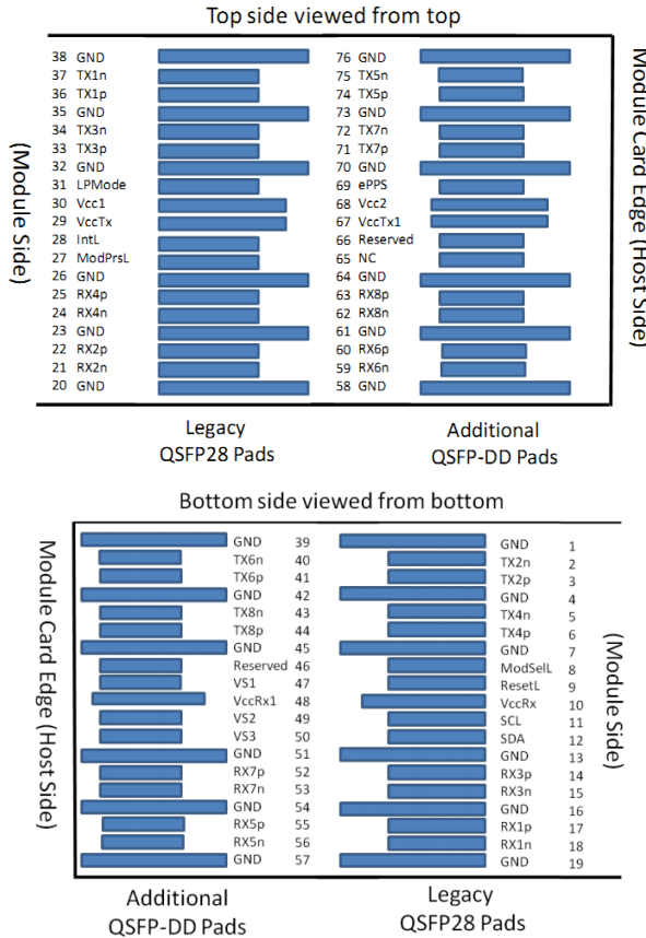
Figure 2, Pin View for QSF-DD
