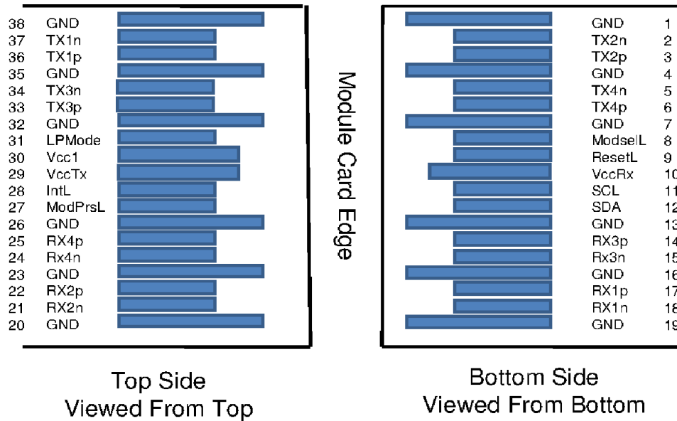
Figure 3, Pin View for QSFP56
