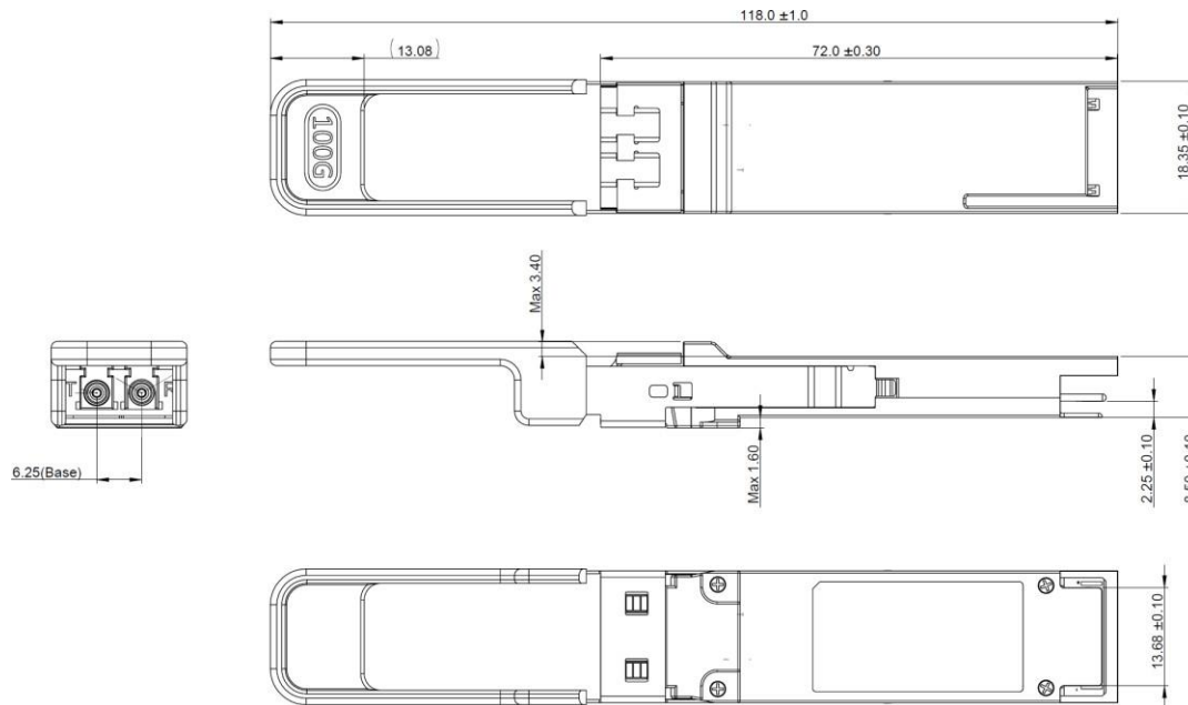
Figure 5. Mechanical Outline
