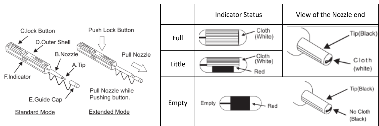
Indicator for remaining cleaning cloth
